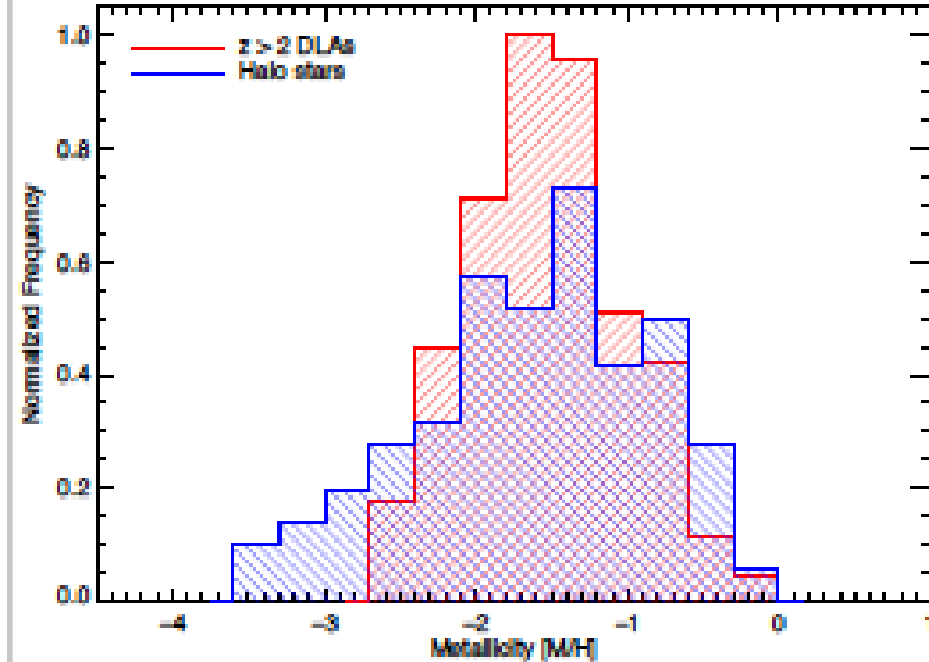
(c) Halo Stars
