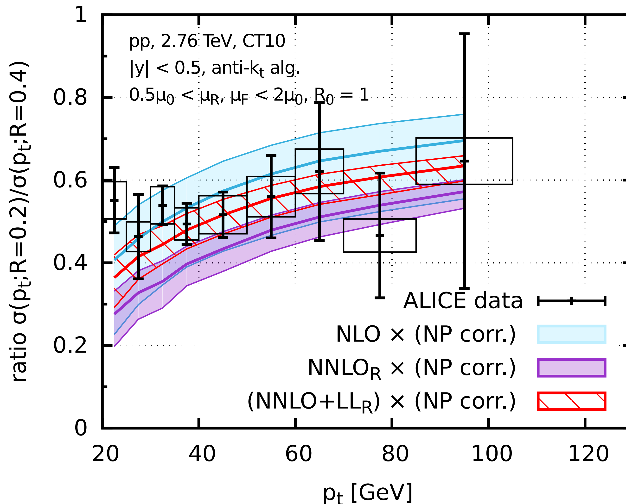
ratio of inclusive jets at R=0.2 and 0.4
